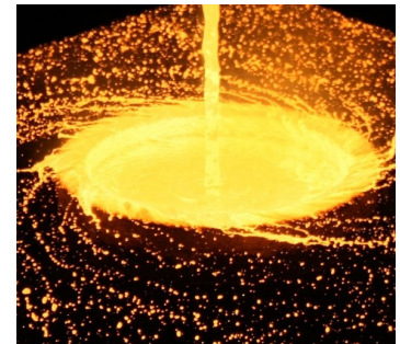
Fe Atomization from Rotating 400mm Disk
