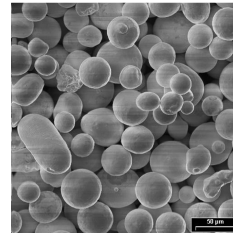
ASL rotary (water quenching)
